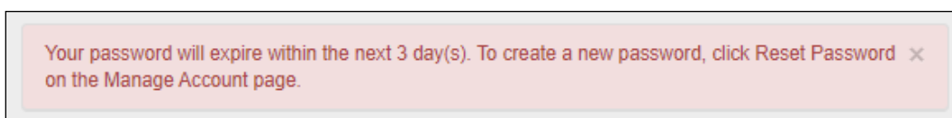
Figure 15. Password Expiration
